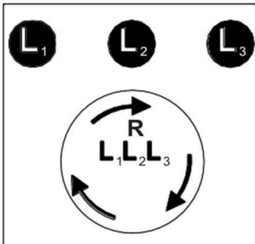
3 phase situation clockwise L1 L2 L3
